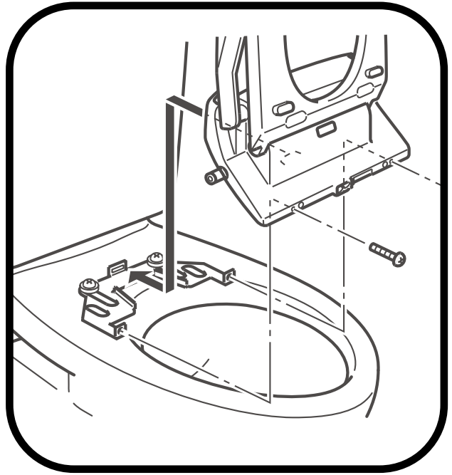
2 Install the seat body.
