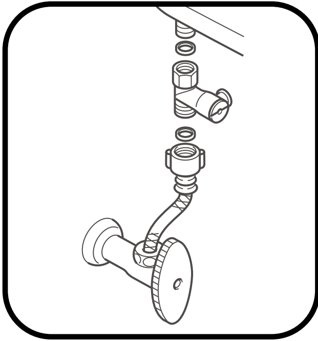
1 Install the junction valve to the water supply.
