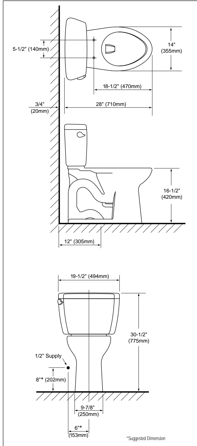
CST744SL - Drake Toilet, ADA Model
