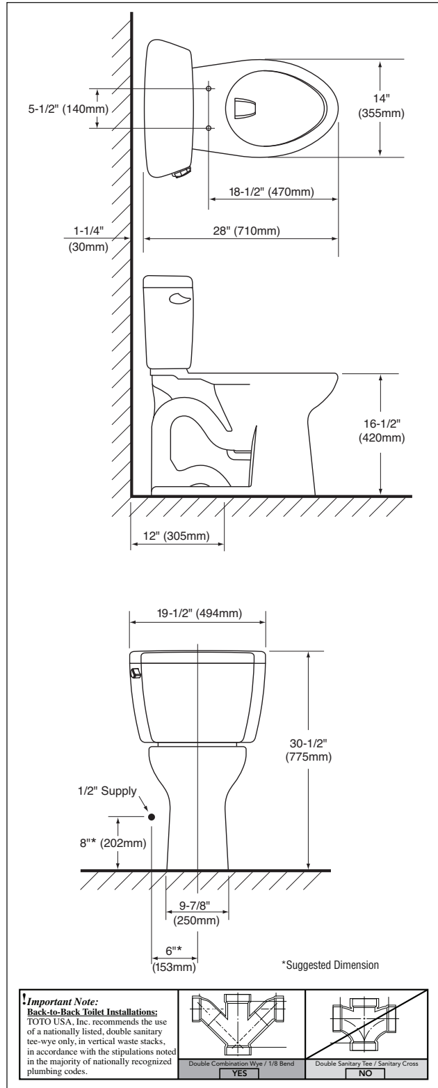
CST744EL - Eco Drake® Close Coupled Toilet
