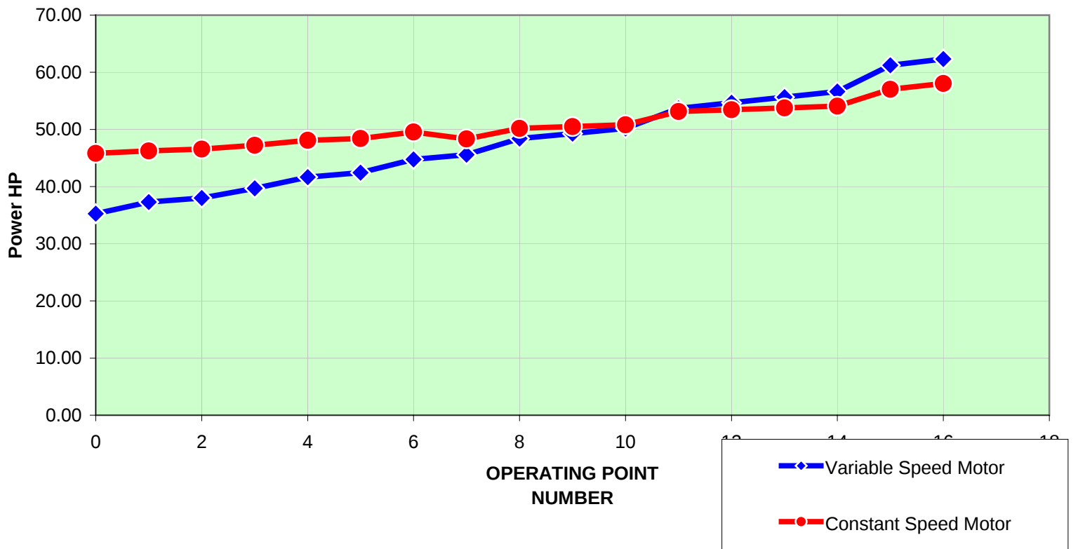
Power Consumption VFD Control vs Constant Speed
